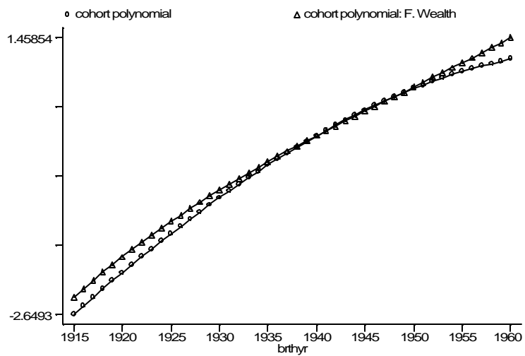
Figure 16: Cohort Effects
