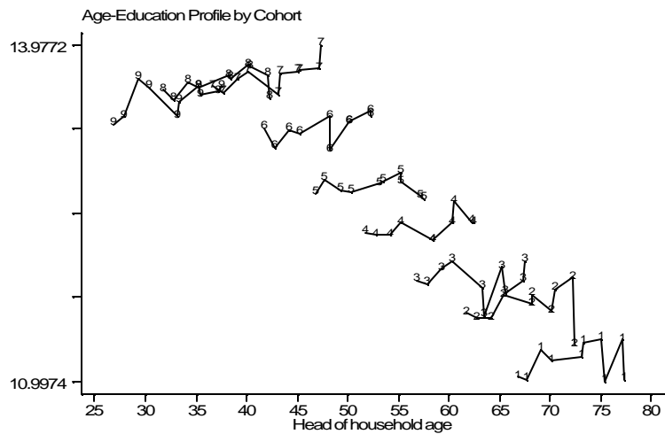
Figure 12: Age-Education Profile
